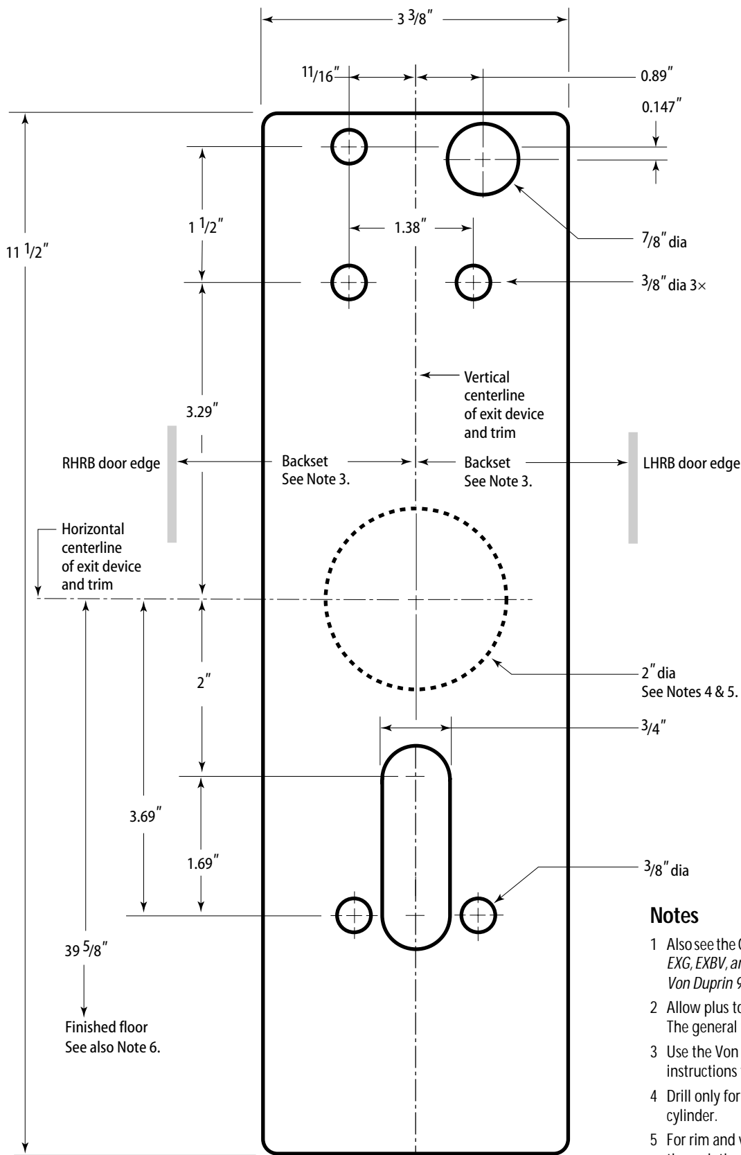
Exit Hardware Trim Escutcheon
