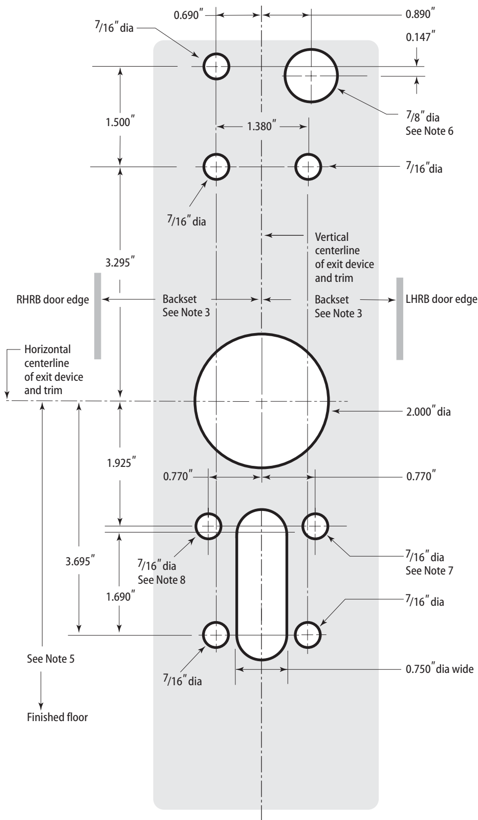
Exit Hardware Trim Escutcheon Footprint (Looking at door from trim side)
